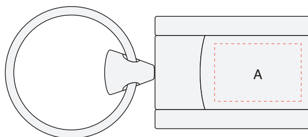
Front Laser Engrave Area A: 22.5mm x 15mm
