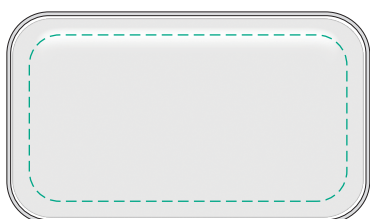
Front Epoxy Dome Plate Size : 46.5 x 26.5 mm Epoxy Dome 4CP Direct Digital Print Image Safe Print Area of 42 x 22 mm
