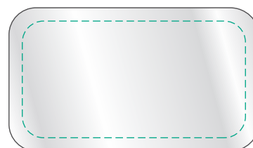
Front Aluminium Plate Plate Size : 46.5 x 26.5 mm Laser Engrave, Pad Print, 4CP Direct Digital Print Image Safe Print Area of 42 x 22 mm
