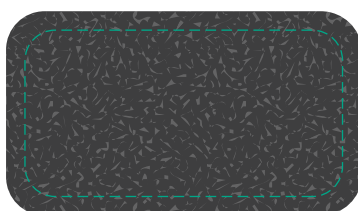
Front PU Leather Plate Size : 46.5 x 26.5 mm Pad Print Deboss Image Safe Print Area of 42 x 22 mm
